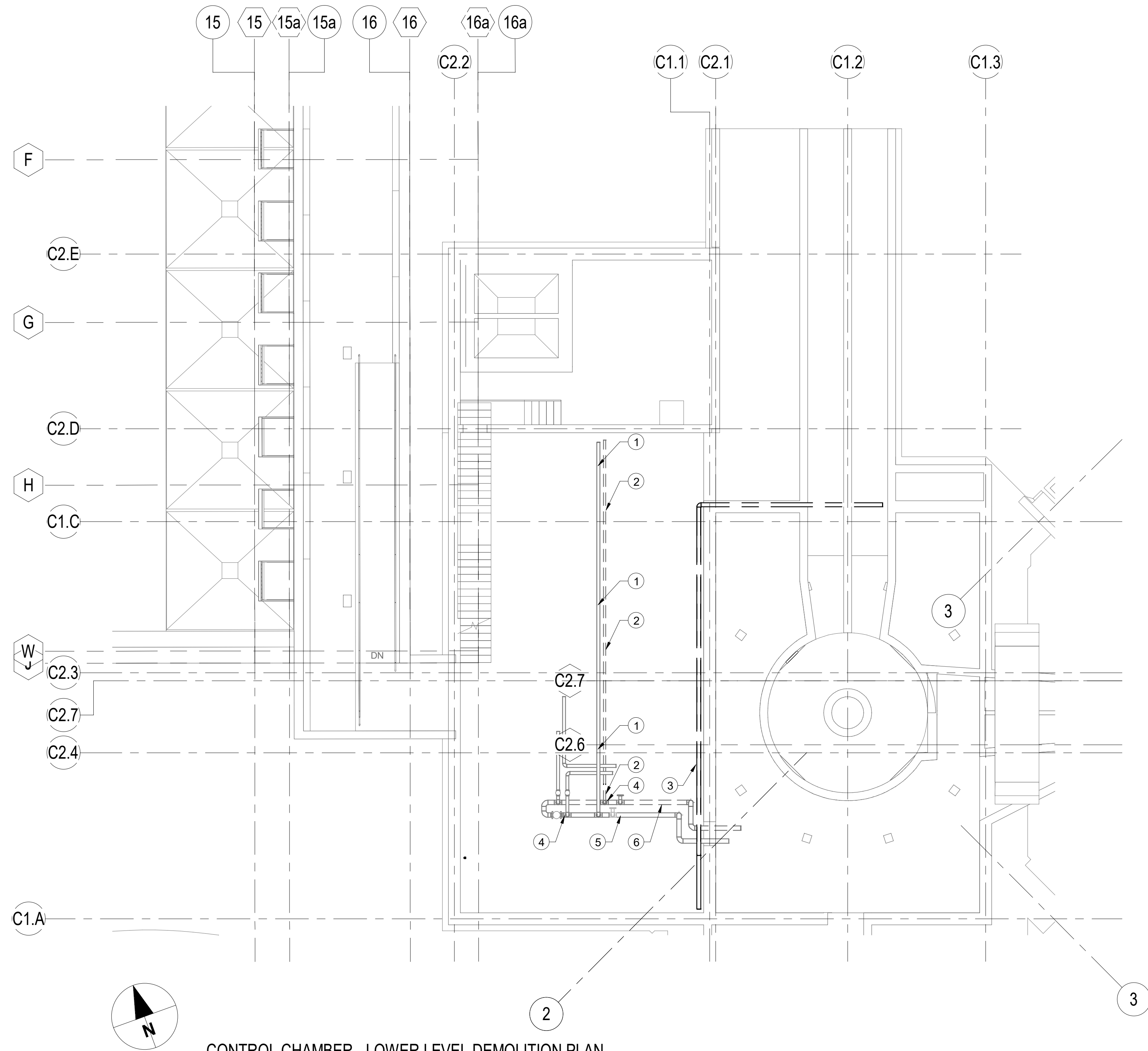
CONTROL CHAMBER - LOWER LEVEL DEMOLITION PLAN SCALE: 1 : 100
